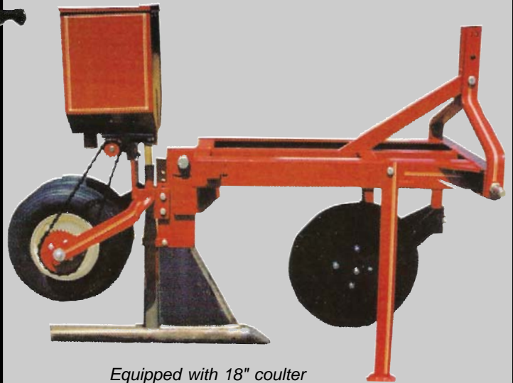
Equipped with 18" coulter
